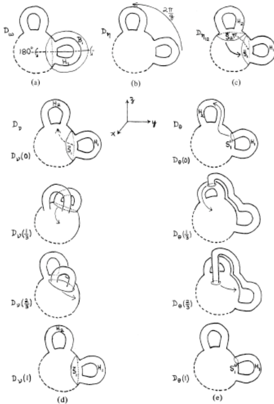
FIGURE 1. Powell's proposed generators
