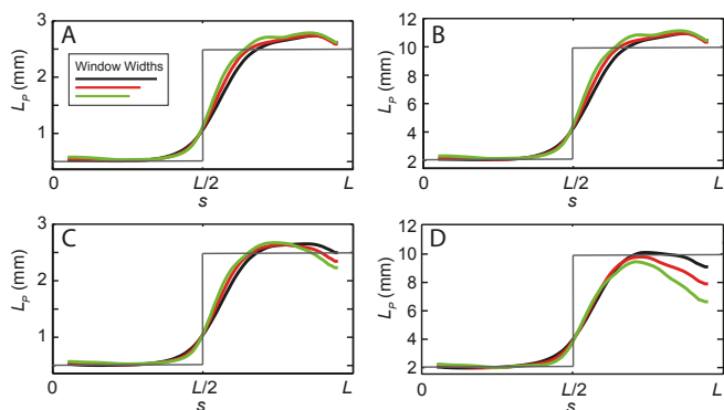
Fig. 2. Validation of Methodology on Simulated Images of Diblock Copolymers, and the Effects of Window Size and Noise. To validate the methodology we show results for the Sliding Window Method for simulated ensembles of contours ( M = 500 ) that are generated with known heterogeneous elasticity (shown in gray). Persistence lengths are determined using three window widths ( L/4 in black, L/5 in red, and L/6 in green). Results for a diblock copolymer, with (A) L_p(0) = 0.5\text{mm} , L_p(L) = 2.5\text{mm} , and no image noise, (B) L_p(0) = 2.5\text{mm} , L_p(L) = 10\text{mm} , and no image noise, (C) L_p(0) = 0.5\text{mm} , L_p(L) = 2.5\text{mm} , and \sigma_b/I_c = 1/6 , and (D) L_p(0) = 2.5\text{mm} , L_p(L) = 10\text{mm} , \sigma_b/I_c = 1/6 are shown.
