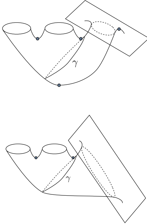
FIGURE 5. Geometrically cancelling the minimum when meeting a type IIIId boundary. Top : Before. Bottom : After.
