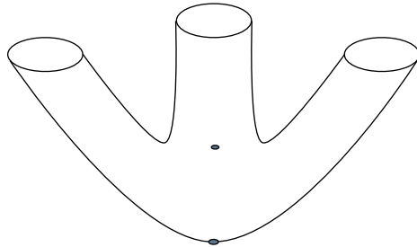
FIGURE 9. A three boundary component genus zero component with one minimum and, instead of two nondegenerate index negative one fixed points, one 3-prong monkey saddle.
