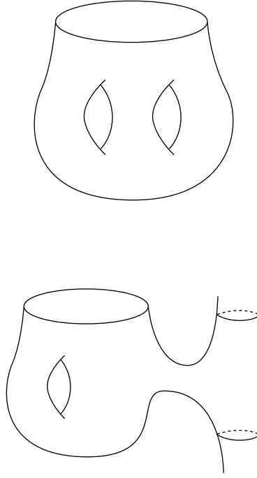
FIGURE 7. On a component which has genus, we can locally cancel the minimum geometrically with an S^1 -valued Hamiltonian. Top: Before. Bottom: After.
